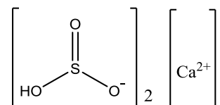
Figure 7: Structural formula of calcium bisulfite
