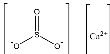
Figure 6: Structural formula of calcium sulfite.
