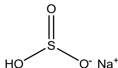
Figure 3: Structural formula of sodium bisulfite.
