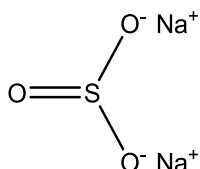
Figure 2: Structural formula of sodium sulfite anhydrous.
