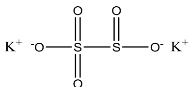
Figure 5: Structural formula of potassium metabisulfite.
