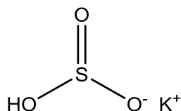
Figure 8: Structural formula of potassium bisulfite
