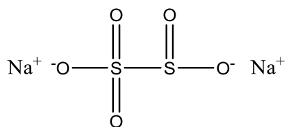
Figure 4: Structural formula of sodium metabisulfite.
