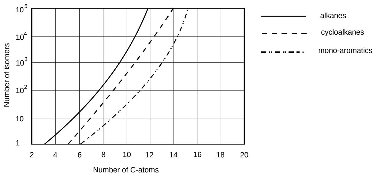
Figure 2: The figure illustrates the possible number of hydrocarbon isomers with a given number of carbon atoms.
